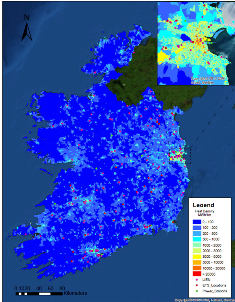
Figure 4-1. Total 2025 Forecast Linear Heat Density (Source: SEAI report 2015)
