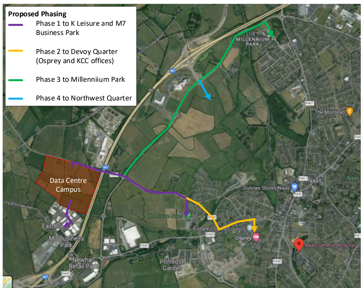
Figure 6-5. Proposed District Heating Network Phasing (Source: Google Maps)
